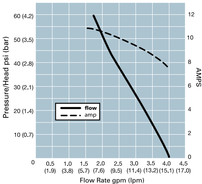
HEAD-FLOW CURVE (12 & 24 VDC)
