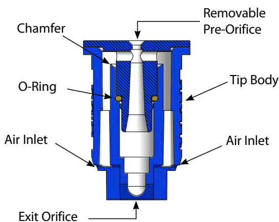
AIXR110 VP Spray Tip (Cross Section View)
